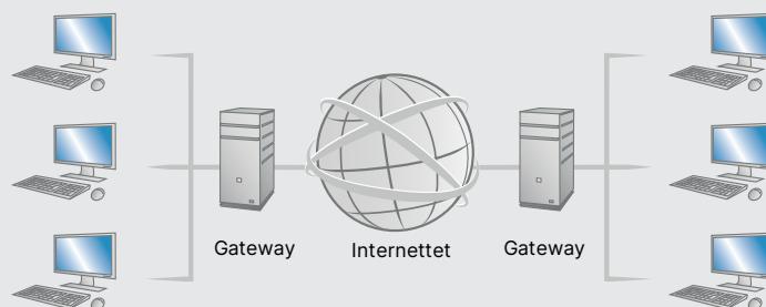
VPN site-to-site
